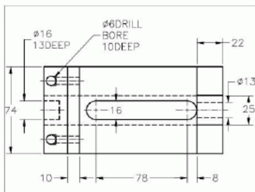
Figure 5 Top view of the Base
