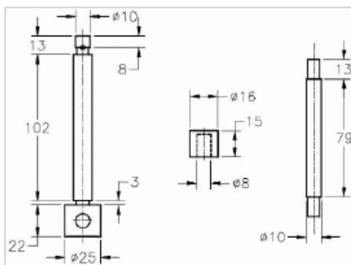
Figure 3 Dimensions of the Clamp Screw, the Handle Stop, and the Clamp Screw Handle
