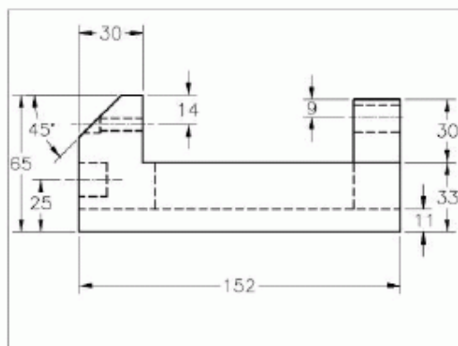
Figure 7 Front view of the Base
