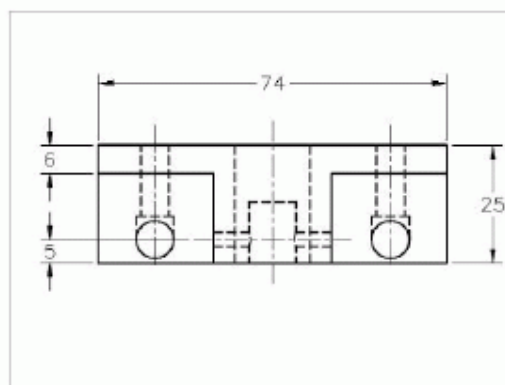
Figure 6 Top view of the Movable Jaw
