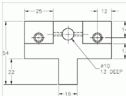
Figure 8 Front view of the Movable Jaw
